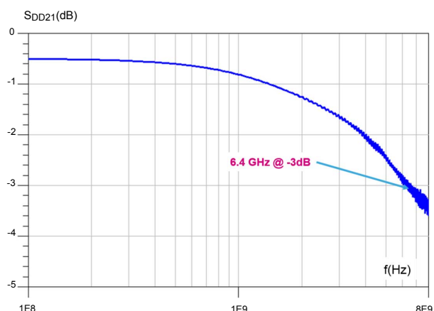
Figure 2. Differential attenuation versus frequency ( Z_{0\text{ DIFF}} = 100\ \Omega )
