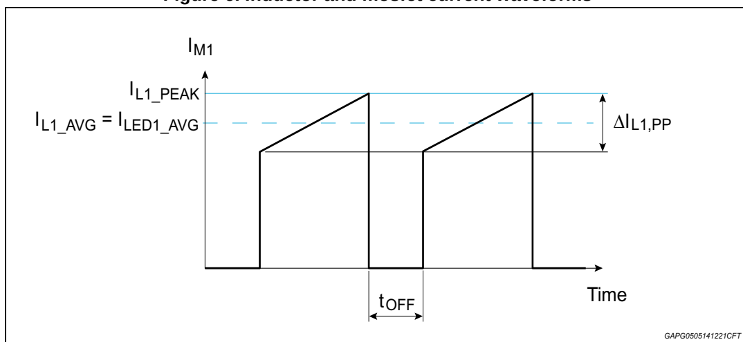
Figure 6. Inductor and mosfet current waveforms
