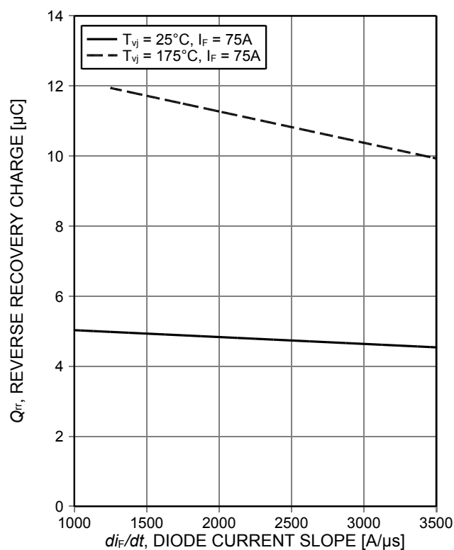
Figure 20. Typical reverse recovery charge as a function of diode current slope ( V_R=600\text{V} )
