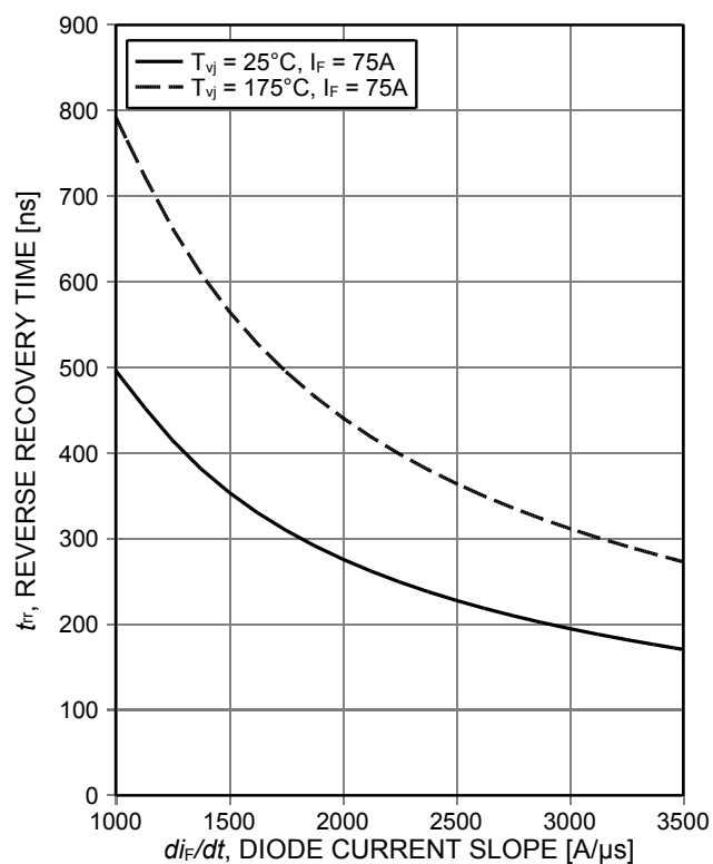
Figure 19. Typical reverse recovery time as a function of diode current slope ( V_R=600\text{V} )
