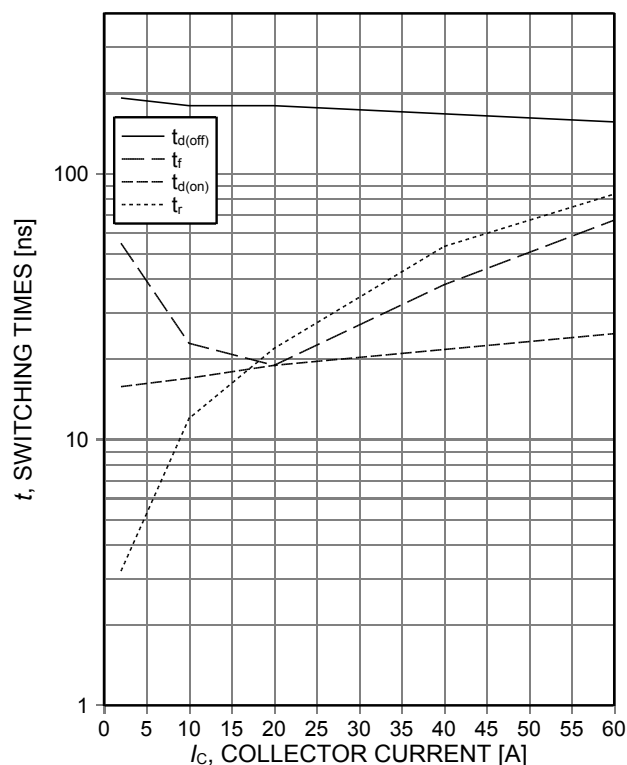
Figure 7. Typical switching times as a function of collector current (inductive load, T_J=150^\circ C , V_{CE}=400V , V_{GE}=0/15V , R_G=32\Omega , Dynamic test circuit in Figure E)
