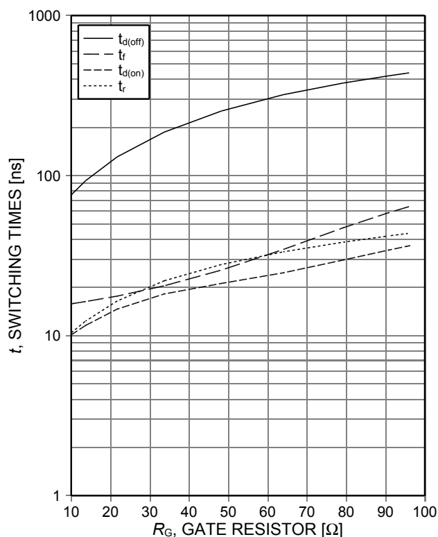
Figure 8. Typical switching times as a function of gate resistor (inductive load, T_J=150^\circ C , V_{CE}=400V , V_{GE}=0/15V , I_C=20A , Dynamic test circuit in Figure E)
