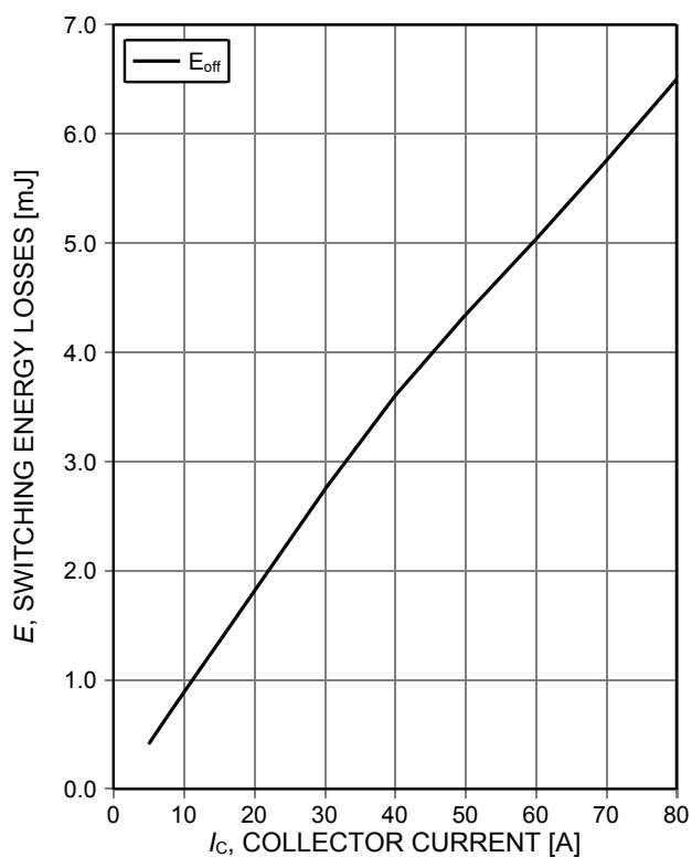
Figure 12. Typical switching energy losses as a function of collector current (inductive load, T_j=175^\circ\text{C} , V_{CE}=600\text{V} , V_{GE}=0/15\text{V} , R_G=10\Omega , Dynamic test circuit in Figure E)
