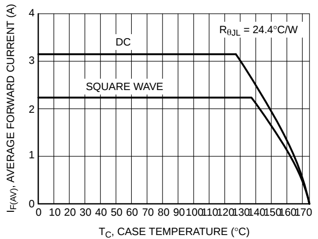
Figure 6. Current Derating
