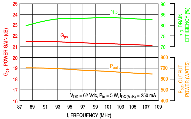
Figure 5. Power Gain, Drain Efficiency and CW Output Power versus Frequency at a Constant Input Power
