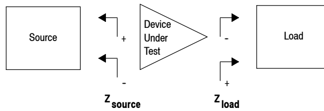
Figure 16. Simulated Source and Load Impedances Optimized for IRL, Output Power and Drain Efficiency — Push-Pull
