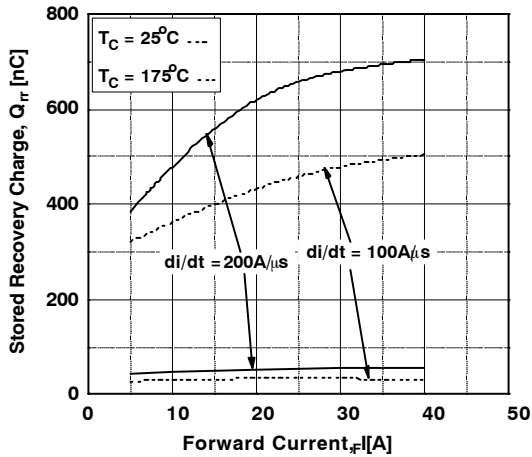
Figure 21. Stored Charge
