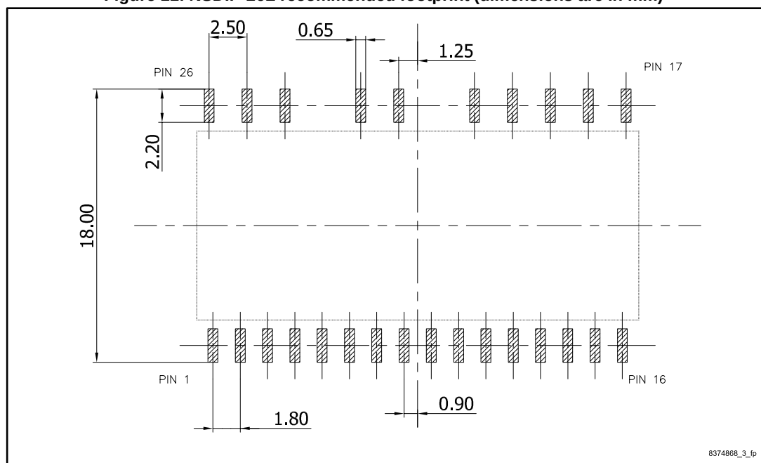
Figure 11: NSDIP-26L recommended footprint (dimensions are in mm)
