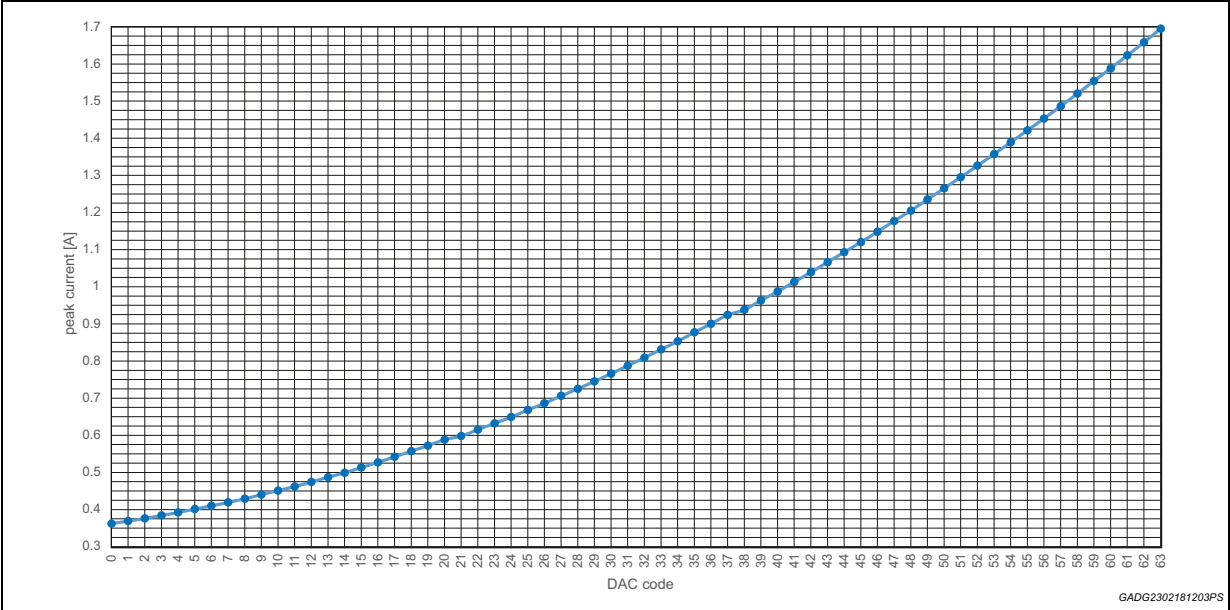
Figure 11. IL_PEAK vs DAC code - Low R_{dson}
