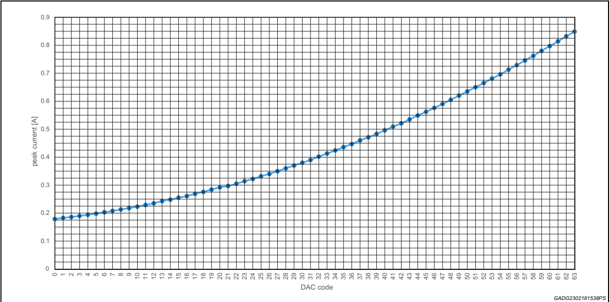
Figure 12. IL_PEAK vs DAC code - High R_{dson}
