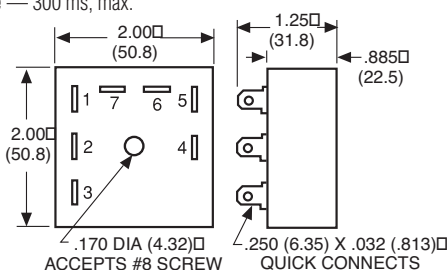
Outline Dimensions
