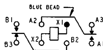
TERMINAL VIEW
