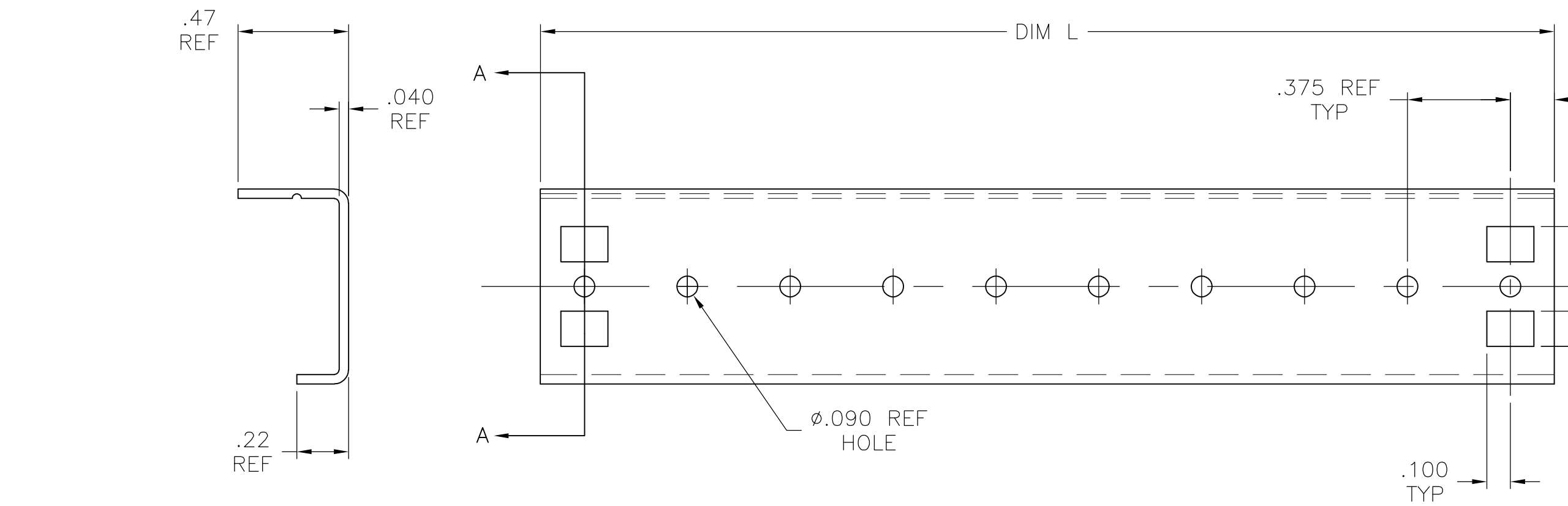
SAFETY COVER QTY 1
