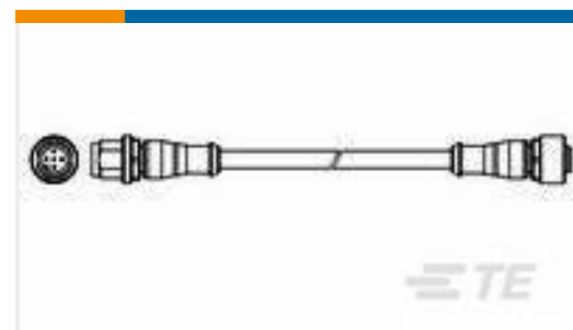
TE Part #2273112-5 M12 strgt plug to M12 strgt socket AA
