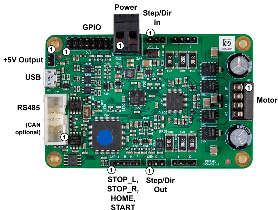
Figure 2: TCM-1316 StepRocker Servo Connectors
