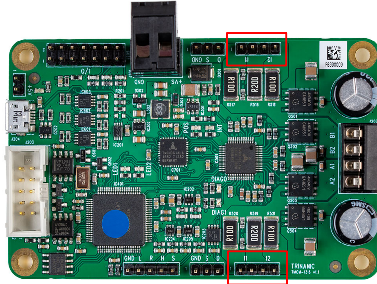
Figure 3: Jumper Settings of the TMC-1316 StepRocker Servo
