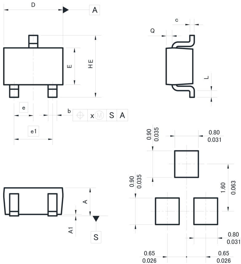
Soldering footprint
