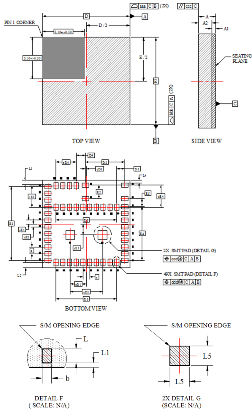
Figure 7.2. BGS13S Package Dimensions
