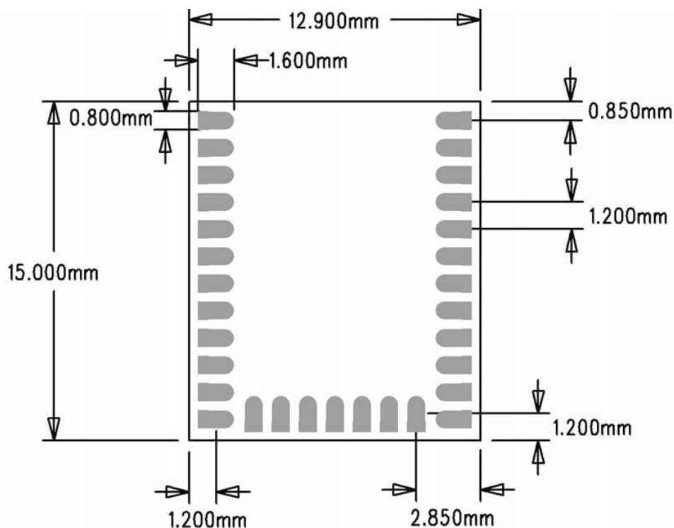
Figure 8.3. BGX13P Footprint
