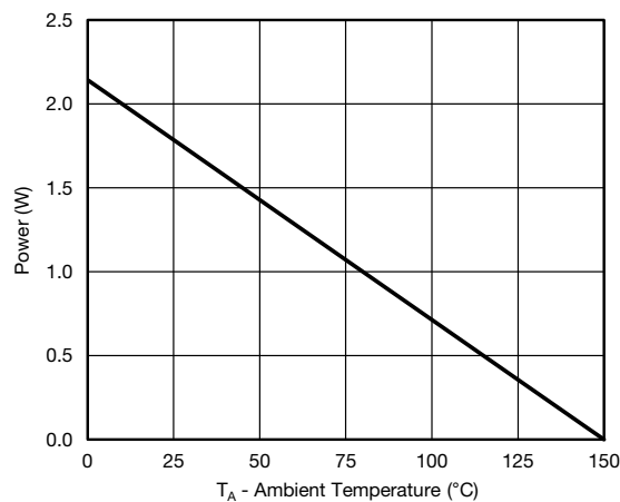
Power, Junction-to-Ambient
