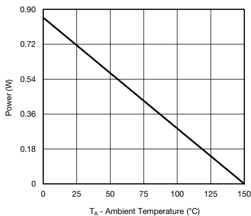
Power, Junction-to-Ambient
