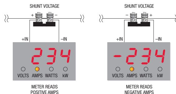
Figure 2. Relationship between shunt voltage polarity and meter reading
