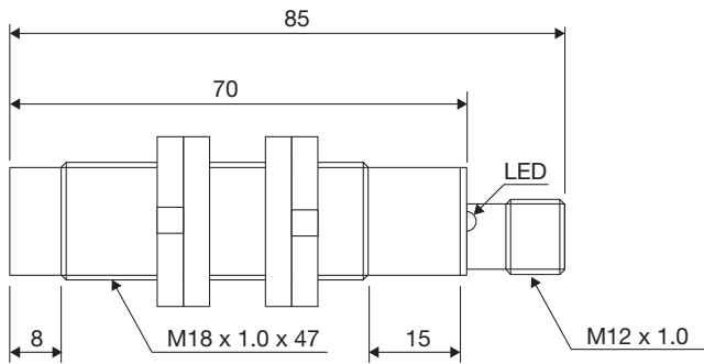
Fig. 9 Plug CA18CAN...M1IO
