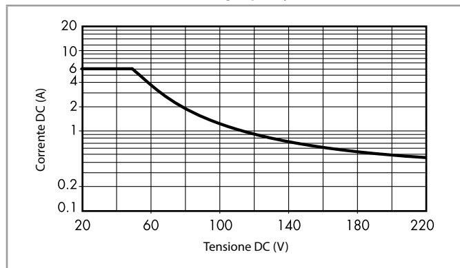
H 7S14* - Maximum DC1 breaking capacity - 7S.14/34
