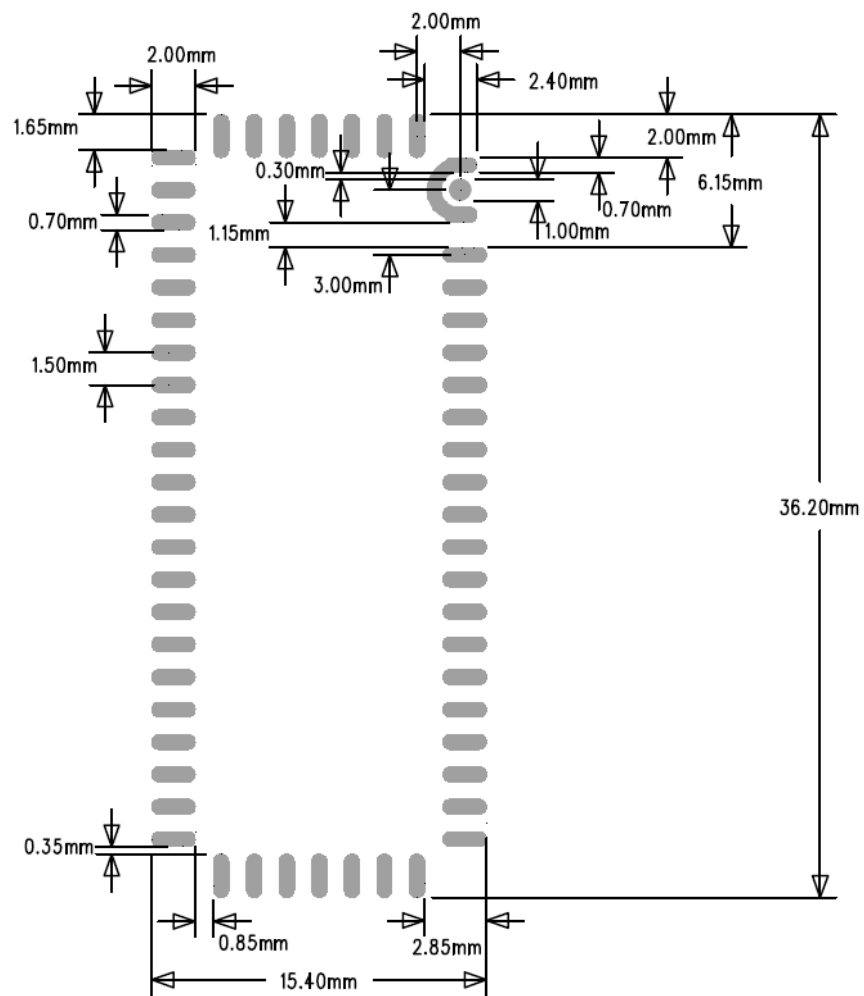
Figure 7: Recommended land pattern
