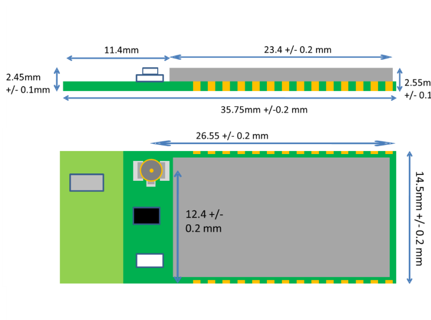
Figure 11: Dimensions of WT11u-E
