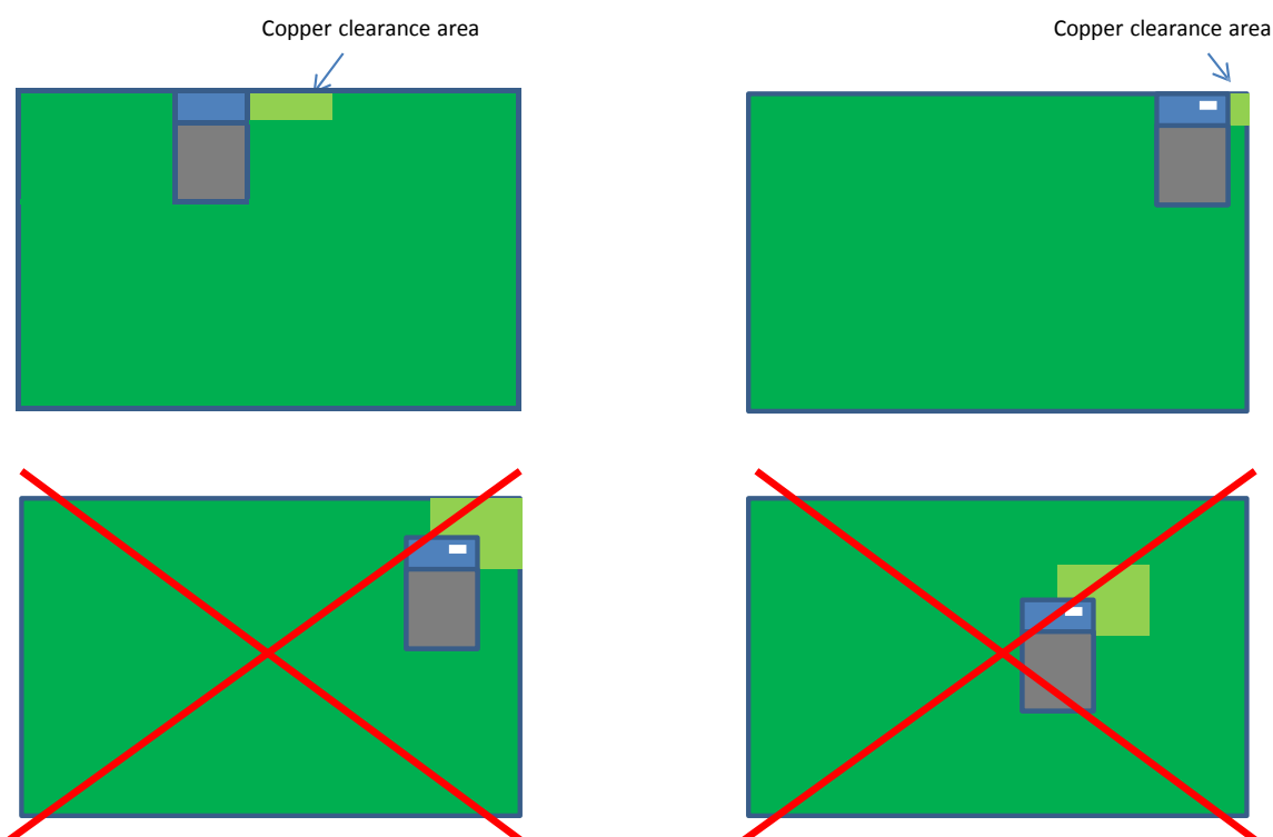
Figure 19: Example layouts for BLE113
