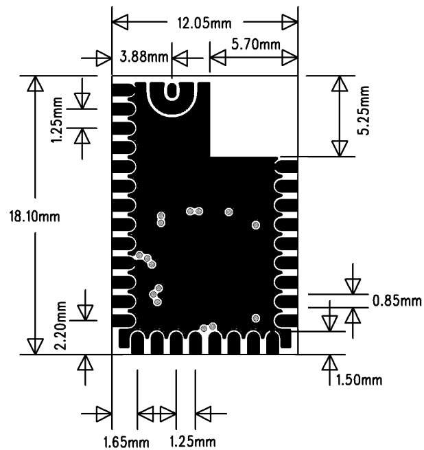
Figure 8: Physical dimensions and pinout (top view)
