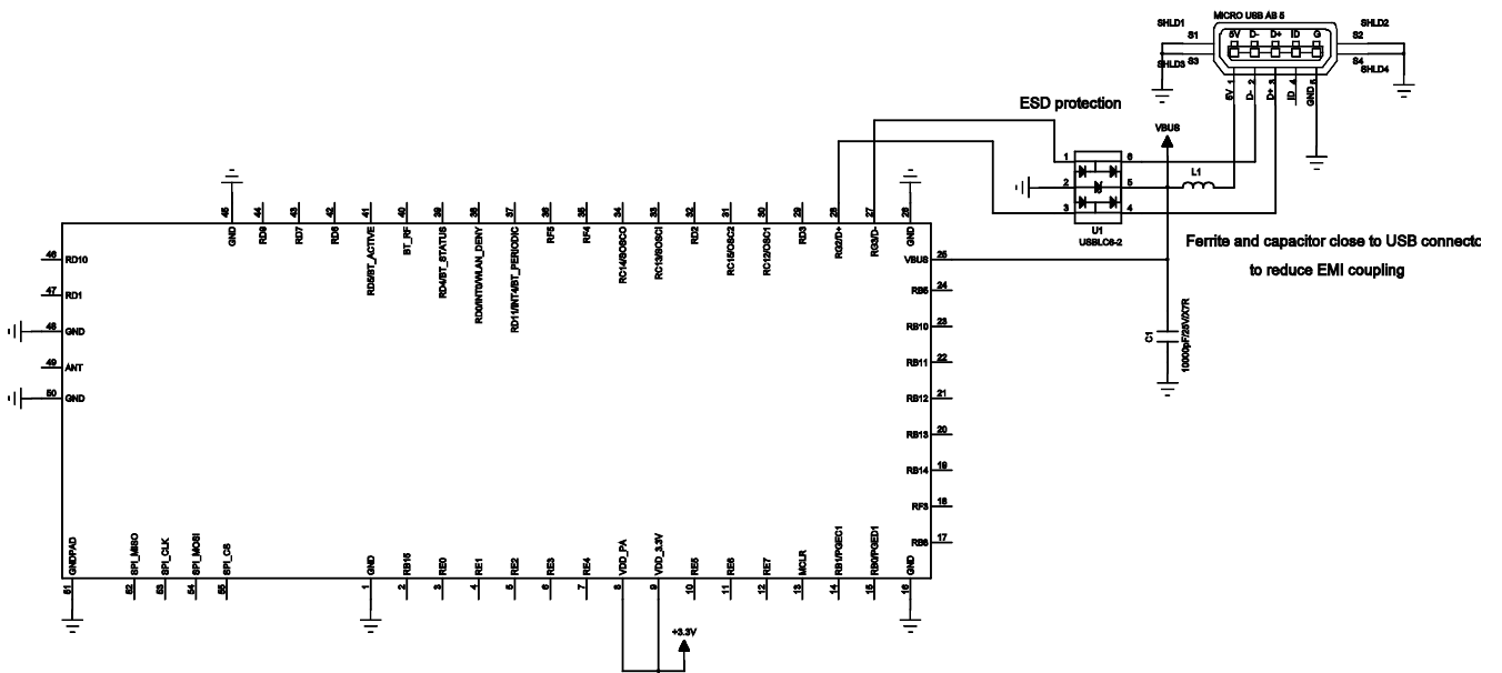
Figure 7: Recommended connections as a USB device. If permanently connected to a hub on the same board, the ESD protection and ferrite can be left out and VUSB can be permanently tied to a supply voltage
