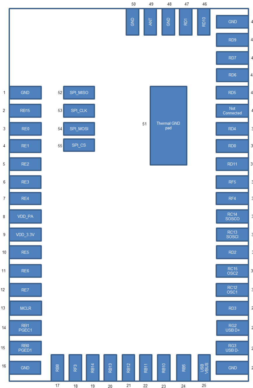
Figure 1: WF121 pinout
