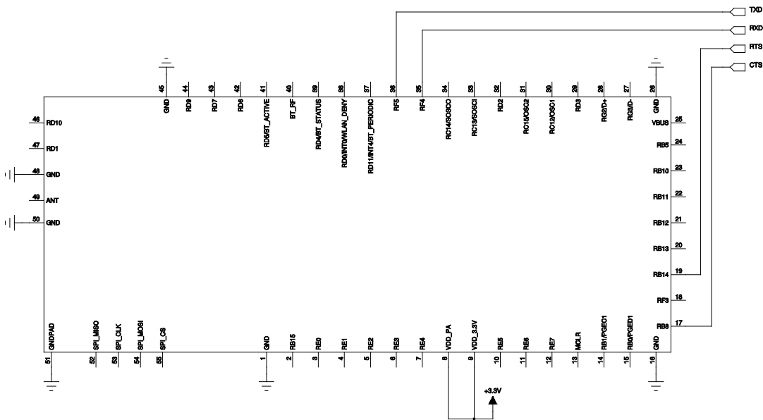
Figure 6: Minimal system required for UART host connection
