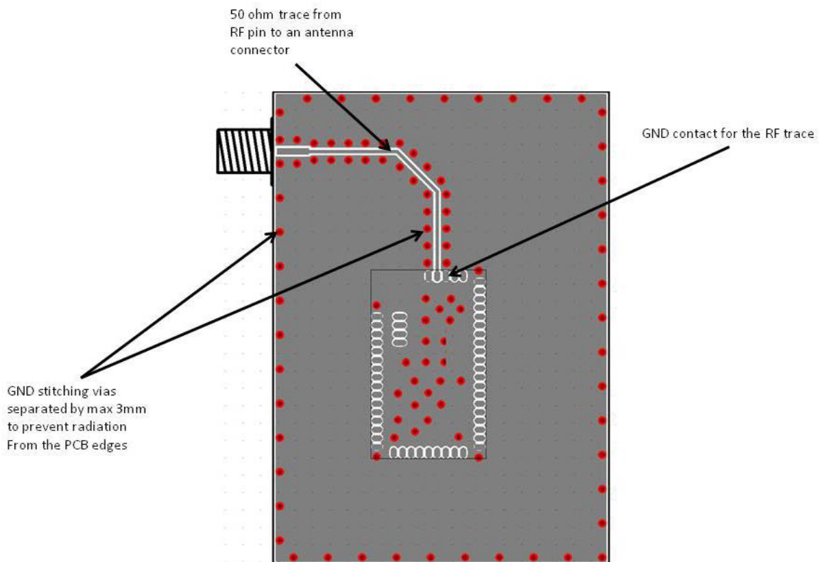
Figure 11: Typical 50 ohm trace from the RF pin to an antenna connector
