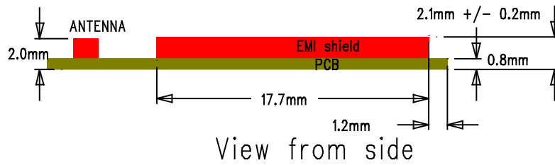
Figure 9: Physical dimensions
