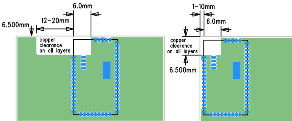
Figure 13: Example layouts, board edge placement on left, board corner on right
