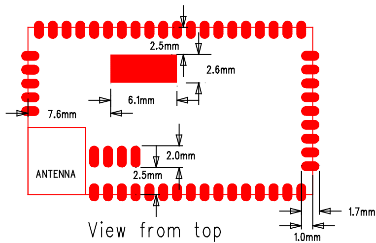
Figure 10: WF121-A recommended PCB land pattern
