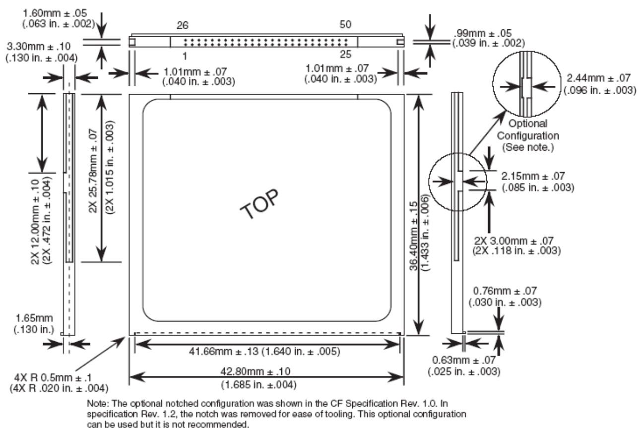
Figure 1. CF Card Dimensions
