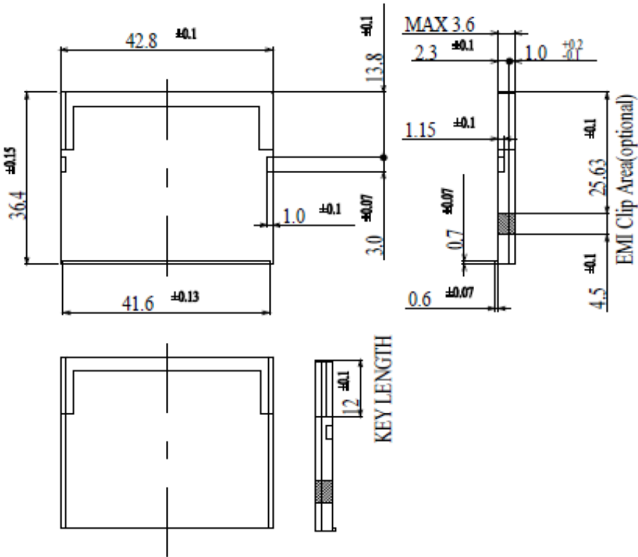
Figure 3. CFast Embedded Module Mechanical Dimensions
