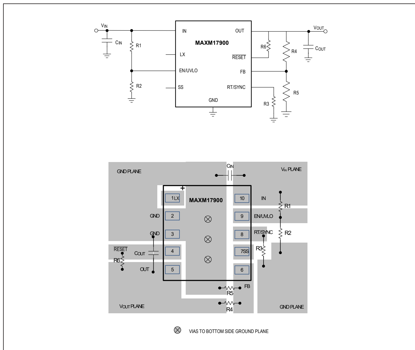
Figure 5. Layout Guidelines
