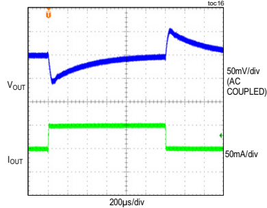
LOAD CURRENT TRANSIENT RESPONSE (V IN = 12V, V OUT = 3.3V, I OUT = 0.05A TO 0.1A)
