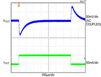
LOAD CURRENT TRANSIENT RESPONSE (V IN = 12V, V OUT = 5V, I OUT = 0A TO 0.05A)
