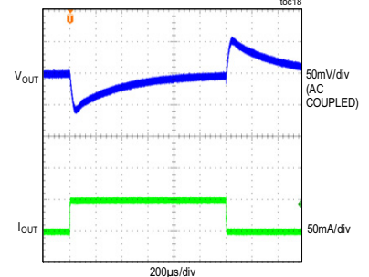
LOAD CURRENT TRANSIENT RESPONSE (V IN = 12V, V OUT = 3.3V, I OUT = 0A TO 0.05A)
