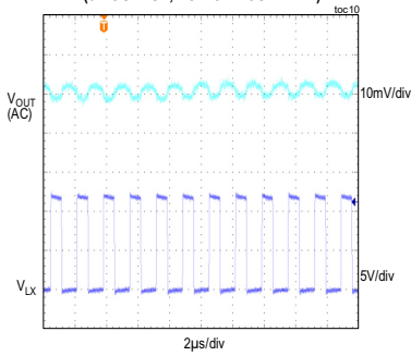
STEADY-STATE SWITCHING WAVEFORMS (5V OUTPUT, NO LOAD CURRENT)
