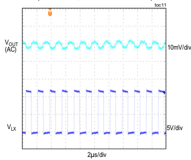
STEADY-STATE SWITCHING WAVEFORMS (5V OUTPUT, 0.1A LOAD CURRENT)
