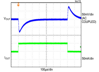
LOAD CURRENT TRANSIENT RESPONSE (V IN = 12V, V OUT = 5V, I OUT = 0.05A TO 0.1A)
