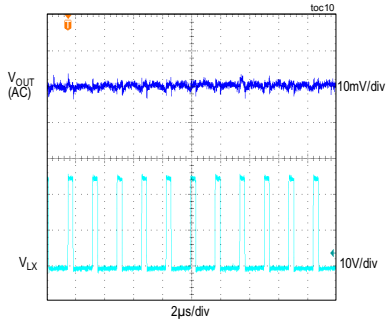
STEADY-STATE SWITCHING WAVEFORMS (5V OUTPUT, NO LOAD CURRENT, PWM MODE)
