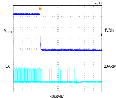
OVERLOAD PROTECTION OUT SHORT TO GROUND
