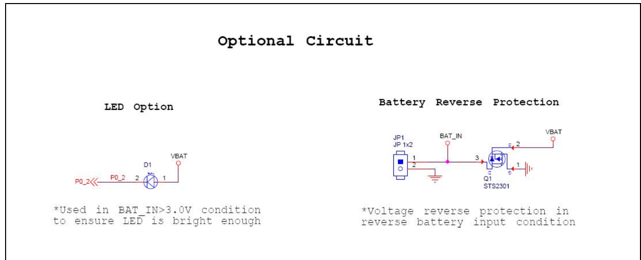
FIGURE 2-4: BM70BLE01FC2 REFERENCE CIRCUIT
