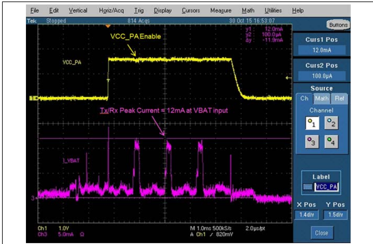
FIGURE 5-1: TX/RX PEAK CURRENT CONSUMPTION OF AN ADVERTISING EVENT
