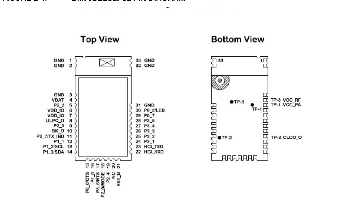
FIGURE 1-4: BM70BLES1FC2 PIN DIAGRAM
