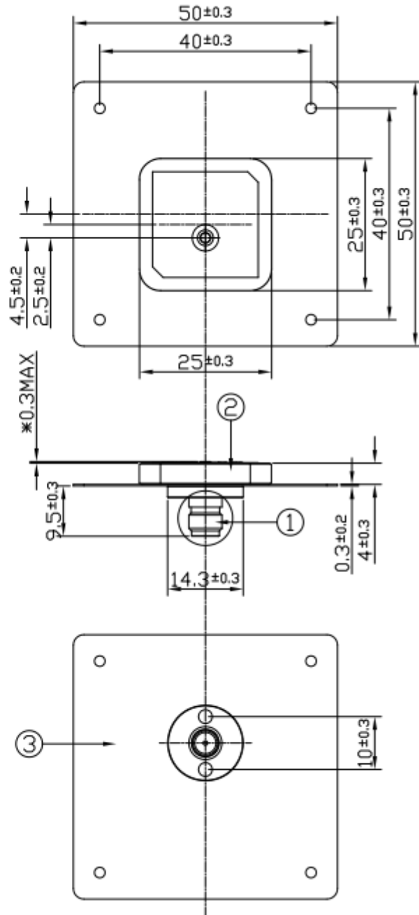
bottom View
