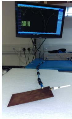
150mm x 90mm Ground Plane
