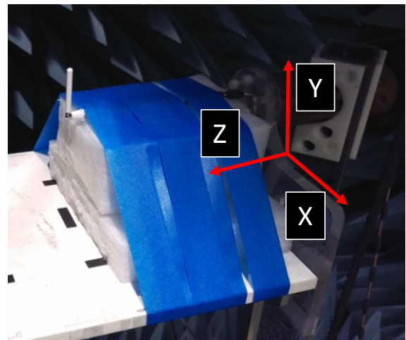
300mm x 300mm Ground Plane Edge
