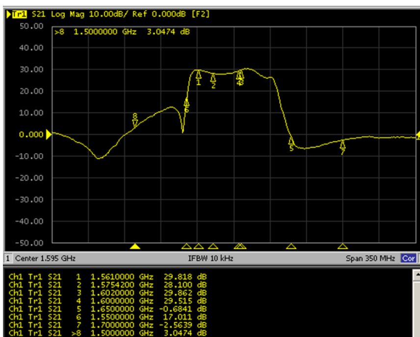
LNA Gain and Out Band Rejection @3.0V
