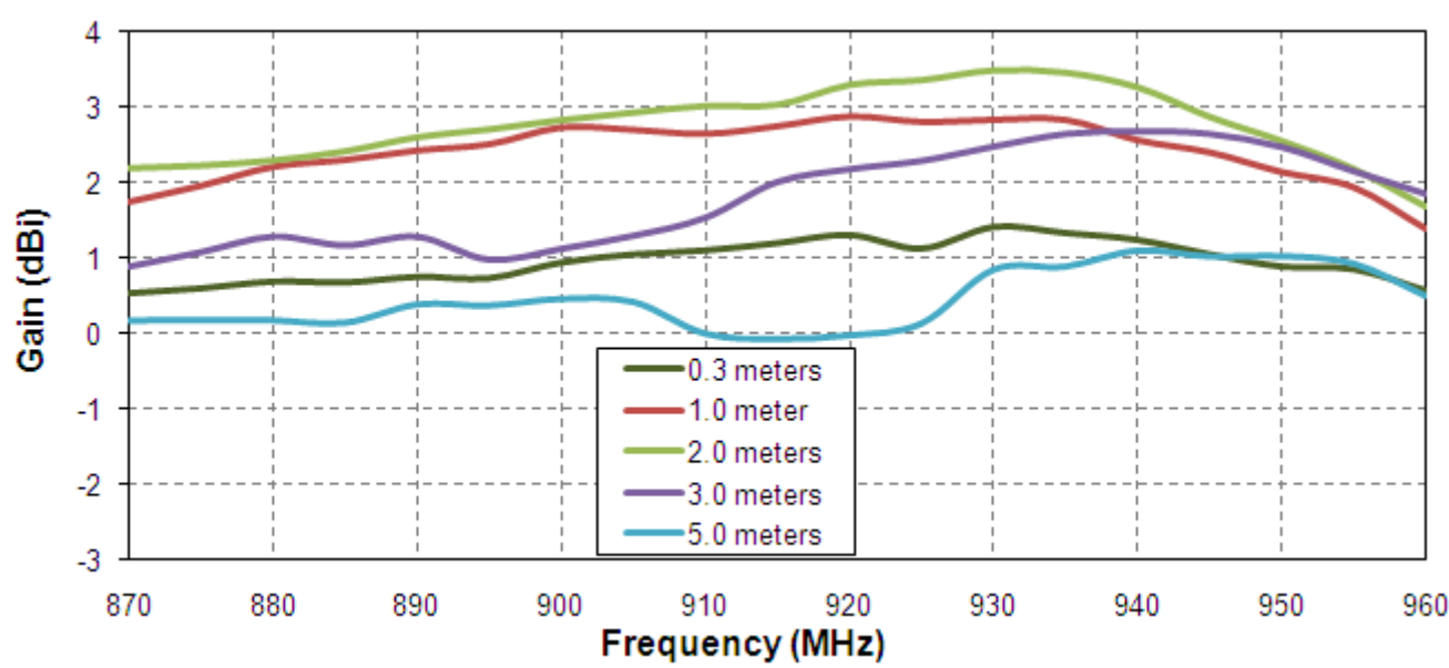
Figure 9. Gain of the 915MHz Hercules ISM antenna on 30 cm metal plate.
