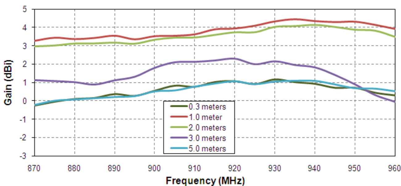
Figure 8. Gain of the 915MHz Hercules ISM antenna in free space.
