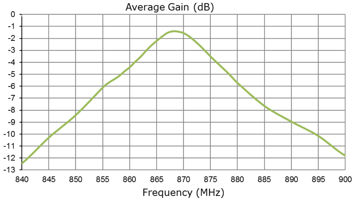
Figure 6. Average Gain of 868 MHz ISM Band Antenna ILA.02
