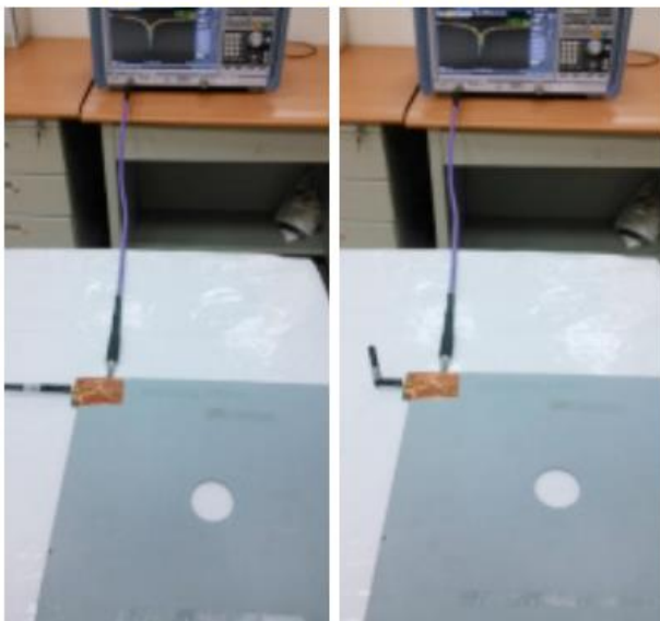
Antenna straight
