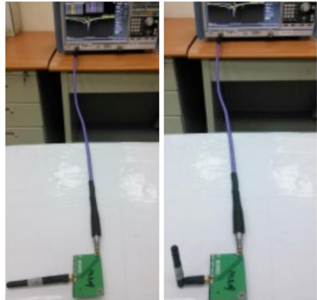
Antenna straight
