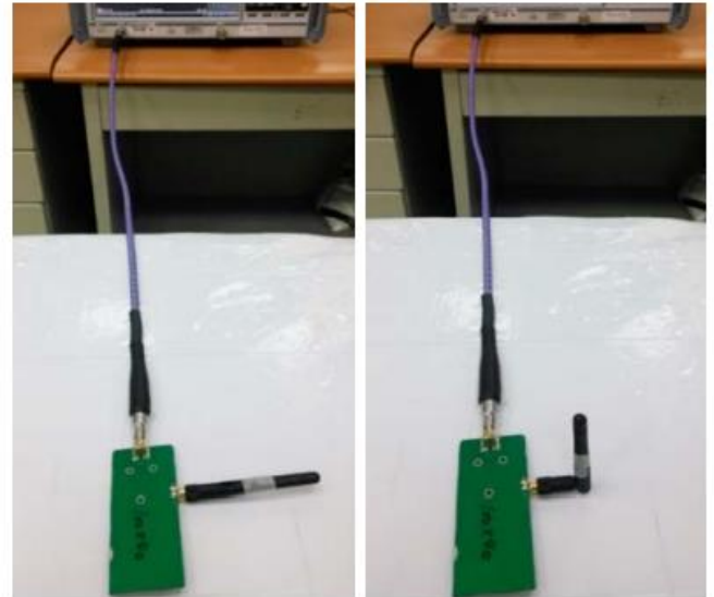
Antenna straight
