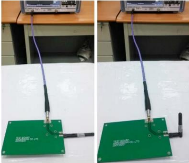
Antenna straight
