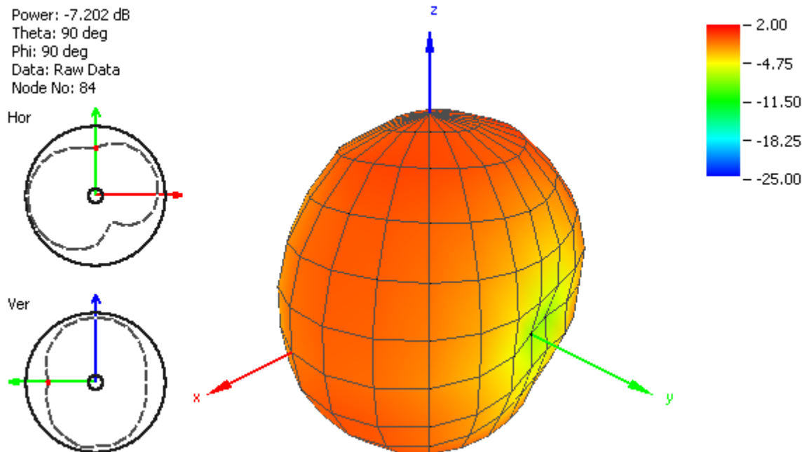
Figure 7. Radiation Pattern at 750 MHz of FXUB66 UWB Antenna.
