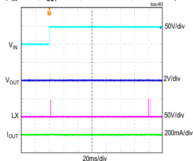
OUTPUT SHORT DURING STARTUP ( V_{IN} = 48V , V_{OUT} = 3.3V , MODE = PWM, FULL LOAD)
