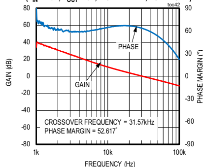
BODE PLOT ( V_{IN} = 48V , V_{OUT} = 5V , MODE = PWM, FULL LOAD)
