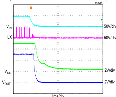
SHUTDOWN THROUGH V_{IN} ( V_{IN} = 48V , V_{OUT} = 5V , PWM MODE, FULL LOAD)
