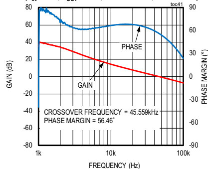
BODE PLOT ( V_{IN} = 48V , V_{OUT} = 3.3V , MODE = PWM, FULL LOAD)
