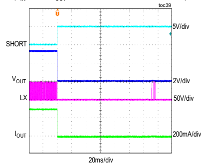
OUTPUT SHORT IN STEADY STATE ( V_{IN} = 48V , V_{OUT} = 3.3V , MODE = PWM, FULL LOAD)
