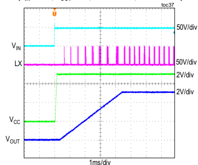
STARTUP THROUGH V_{IN} ( V_{IN} = 48V , V_{OUT} = 5V , PWM MODE, FULL LOAD)
