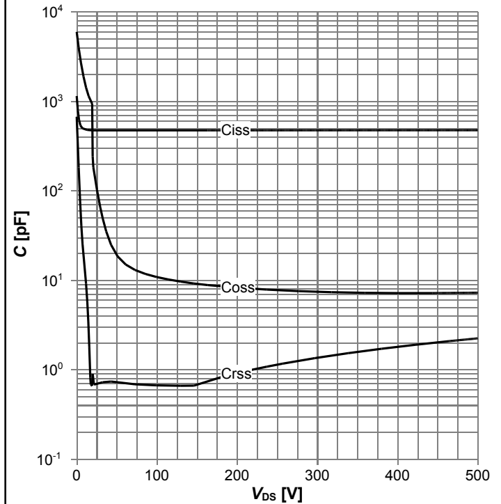
Diagram 14: Typ. capacitances
