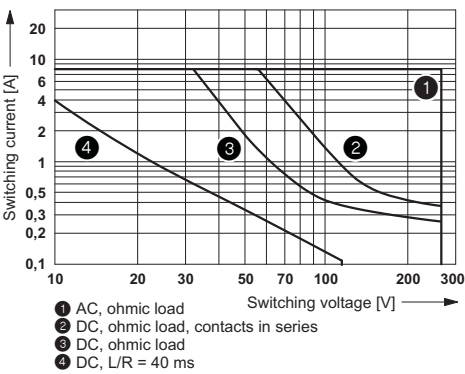
Interrupting rating
