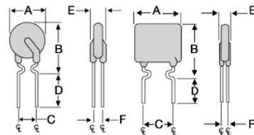
Fig.1 Lead Size :24AWG Ø0.51 mm Diameter
