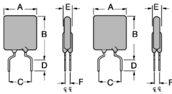
Fig.3 Lead Size : 20AWG Ø 0.81 mm Diameter
