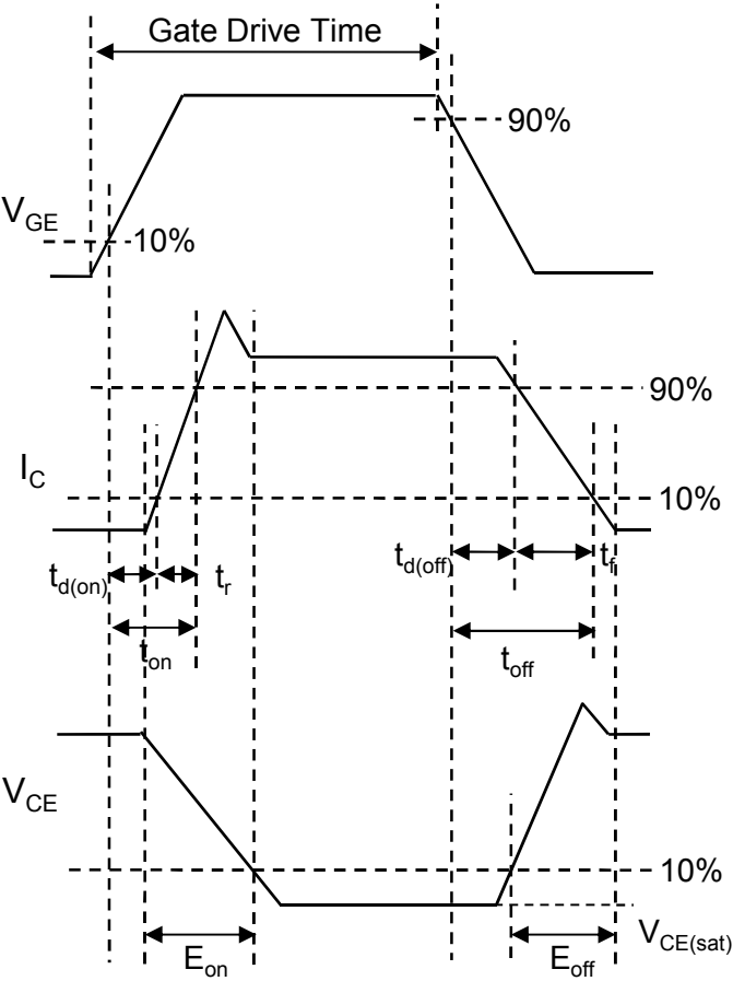
Fig.19 Inductive Load Waveform
