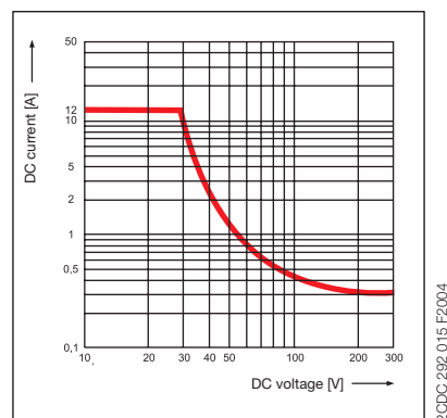
Versions with 2 c/o contacts (CR-M ... 2)
