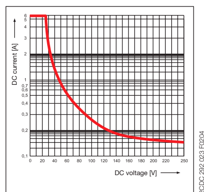
Versions with 4 c/o contacts (CR-M ... 4)
