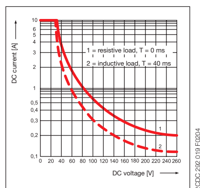
Versions with 3 c/o contacts (CR-M ... 3)
