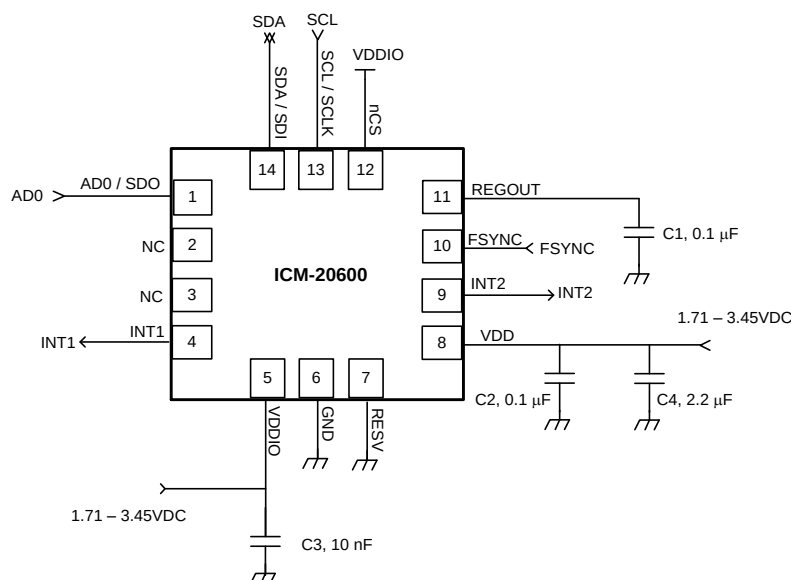
Figure 4. ICM-20600 LGA Application Schematic (I²C Operation)
