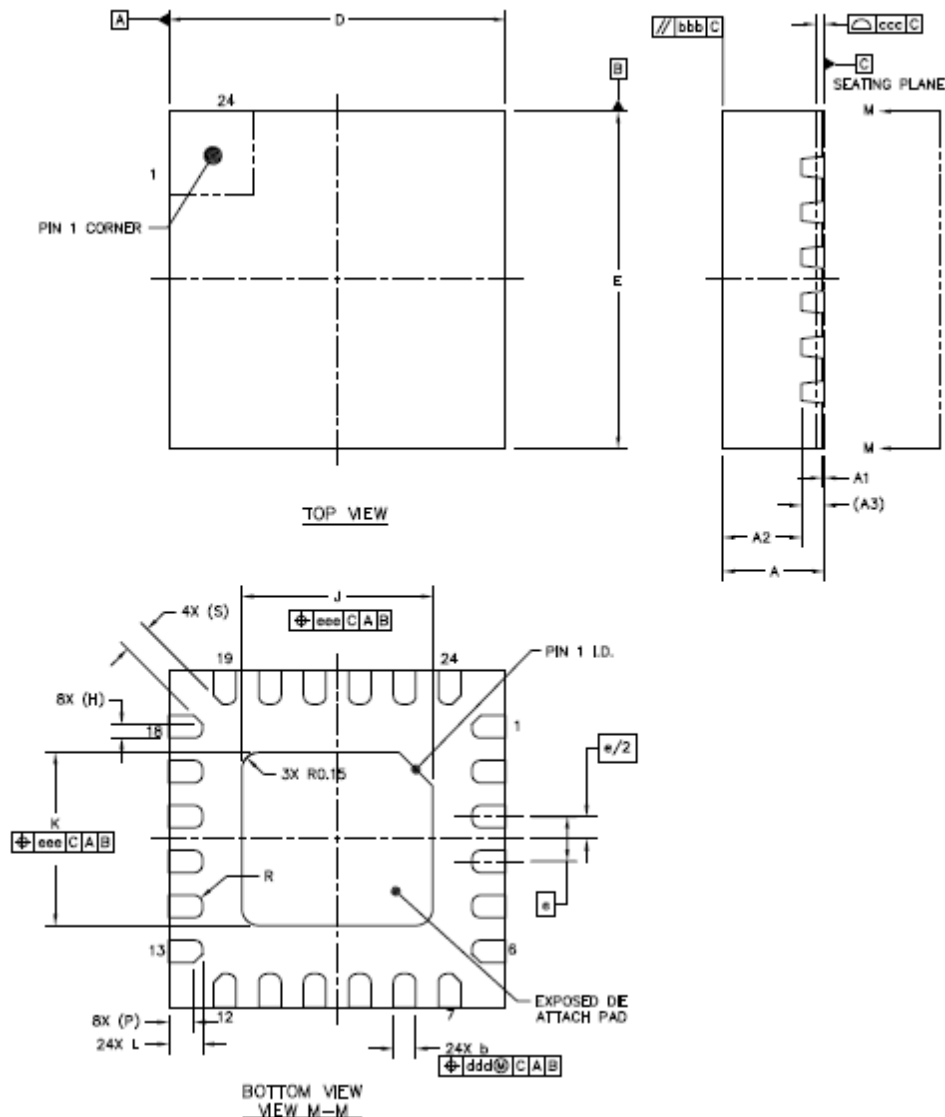
Figure 14. Package Dimensions
