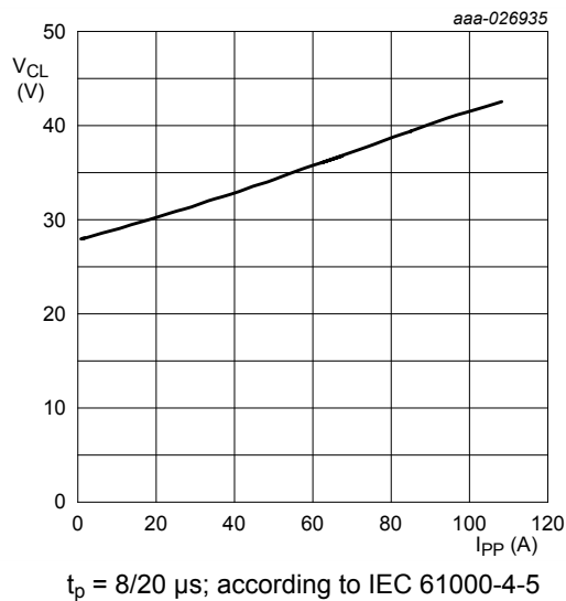
Fig. 8. Positive clamping voltage (8/20 \mu s pulse); typical values
