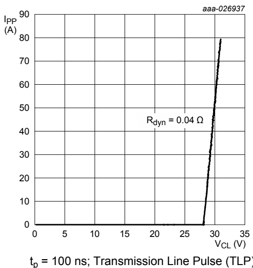
Fig. 10. Dynamic resistance with positive clamping voltage; typical value
