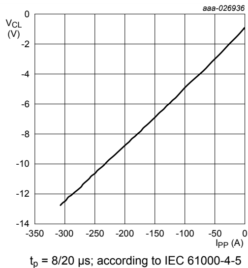
Fig. 9. Negative clamping voltage (8/20 \mu s pulse); typical values
