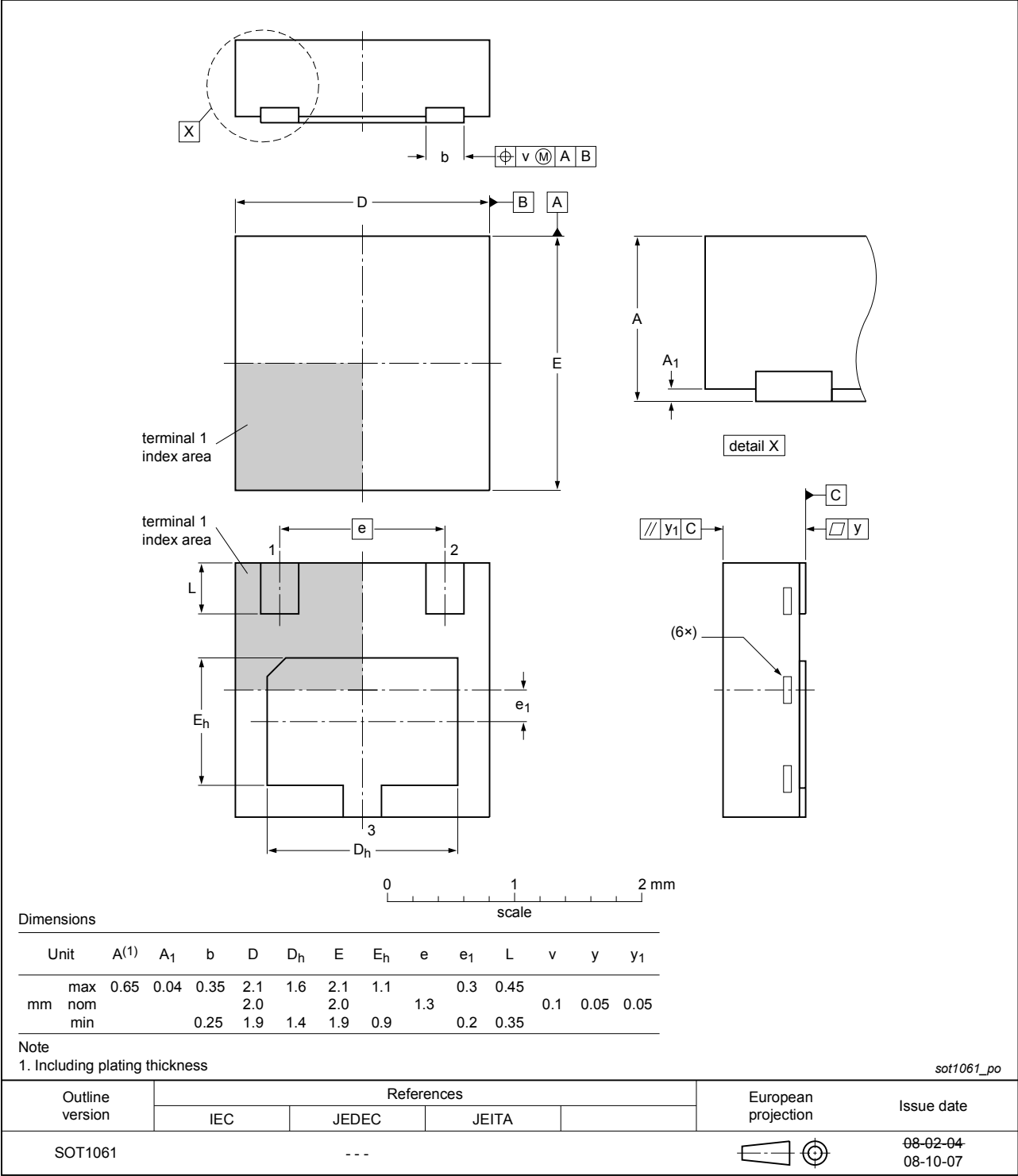
Fig. 16. Package outline DFN2020-3 (SOT1061)
