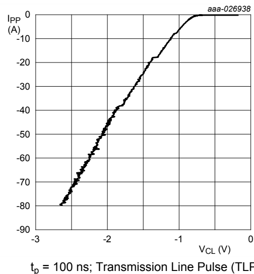
Fig. 11. Dynamic resistance with negative clamping voltage; typical value
